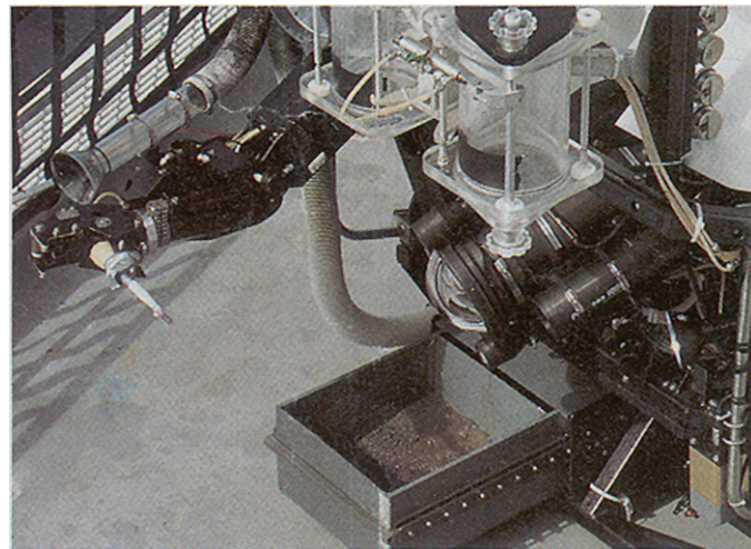
BRUCE H. ROBISON The front of Ventana's frame supports cameras, sensors, samplers and a mechanical arm.
